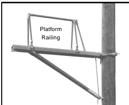
Standard Platform w/ Railing Epoxiglas ® Railing must be ordered as separate item.
