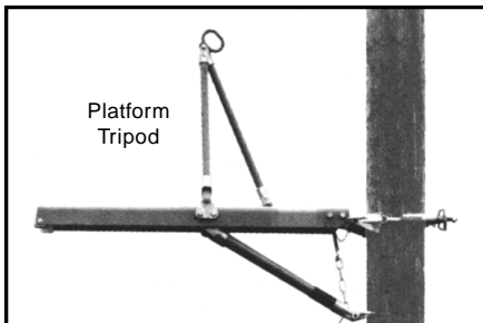
4-ft. Standard Aerial Platform Epoxiglas Tripod must be ordered as separate item.
