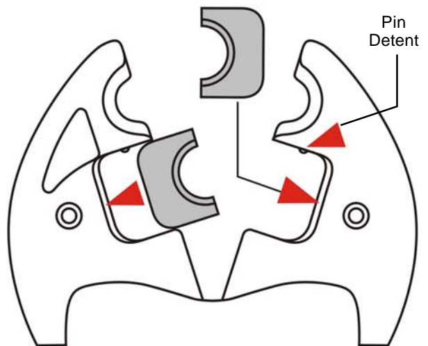
C. R6/W Die Installation with Kearney D3 Nest Die
