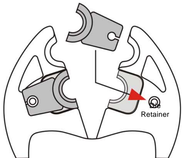
C. R6/W Die Installation with Kearney D3 Nest Die
